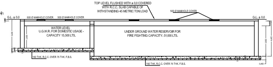
SECTION THROUGH A - A' SCALE 1:50
