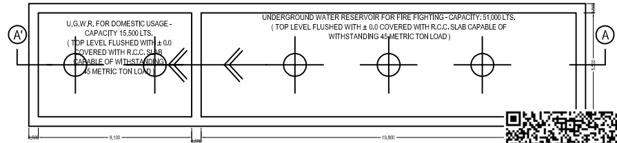
PLAN OF UNDERGROUND WATER RESERVOIR FOR FIRE FIGHTING - CAPACITY 51,000 L. & UNDERGROUND WATER RESERVOIR FOR DOMESTIC USAGE - CAPACITY 15,500 L. SCALE 1:50
